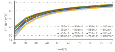
Efficiency VS Load
